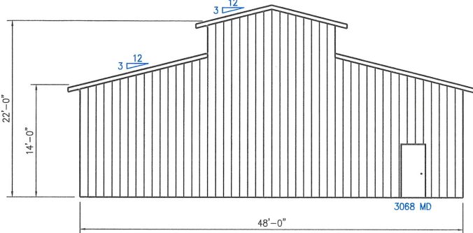
LEFT GABLE VIEW
