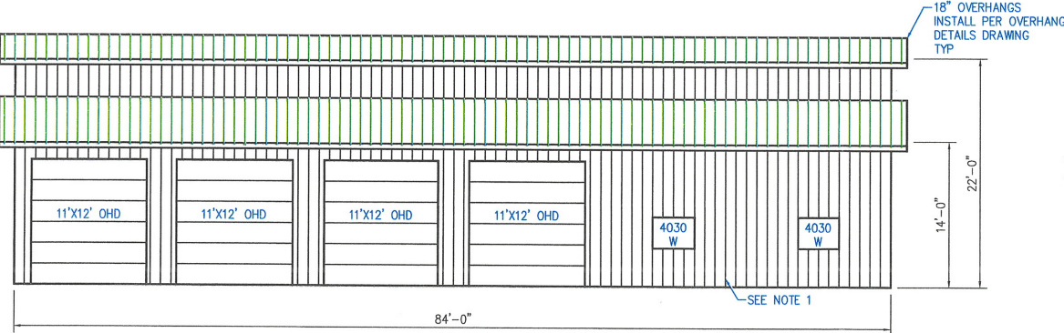
FRONT EAVE VIEW
