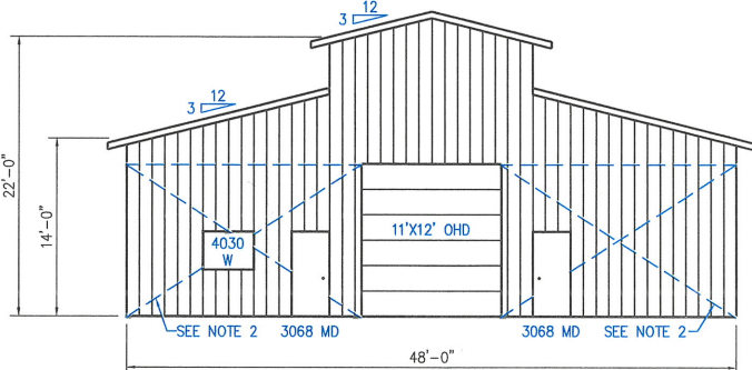
RIGHT GABLE VIEW
